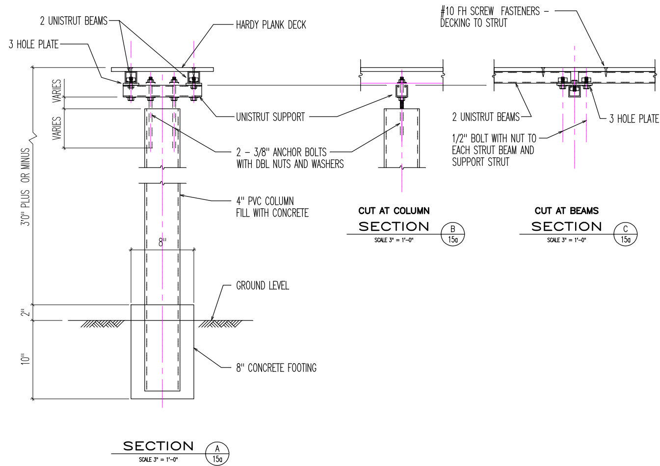
BOLTED TOGETHER STRUT ASSEMBLY 15a
