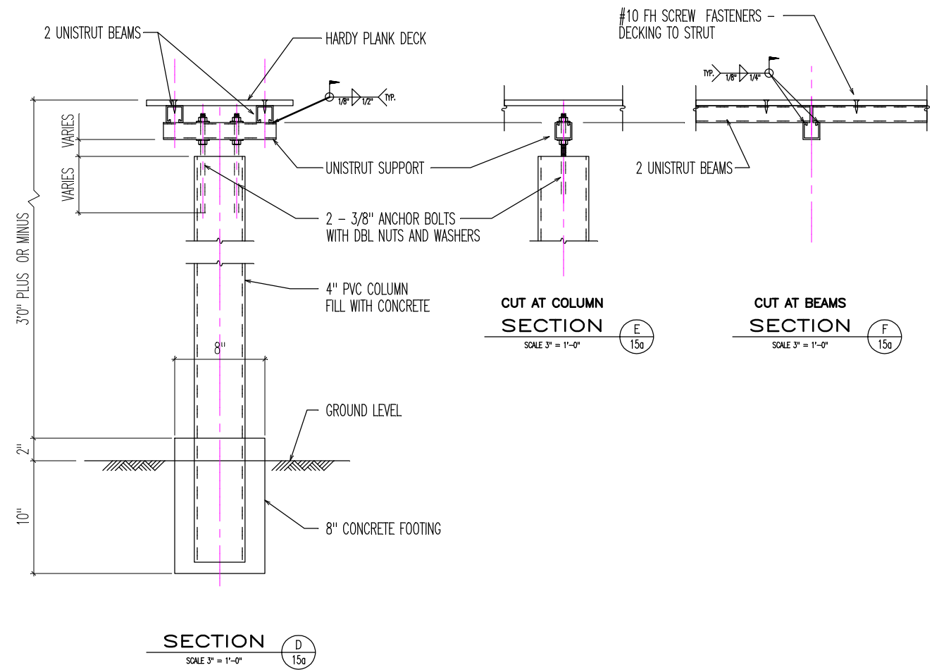
BOLTED / WELDED TOGETHER STRUT ASSEMBLY 15a
